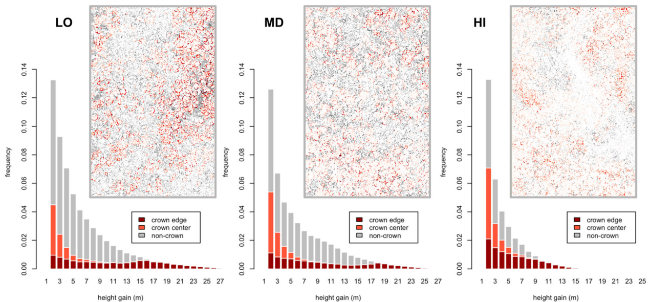
Figure 3. In each 16-ha focus area (LO, MD, HI), 2018 and 2020 canopy tree crown objects (see Figure 2) were used to quantify the distributions of post-hurricane height gains (2018–2020) within crown objects (“crown center”, light red), adjacent to crown objects (“crown edge”, dark red), or associated with shorter vegetation (“non-crown”, gray). Height growth attributed to vertical gains within the horizontal extent of existing crown objects in 2018 (“crown centers”) was primarily \leq 4 m during this interval in all three focus areas (85.1%, 88.3%, and 89.3% for LO, MD, HI, respectively).
