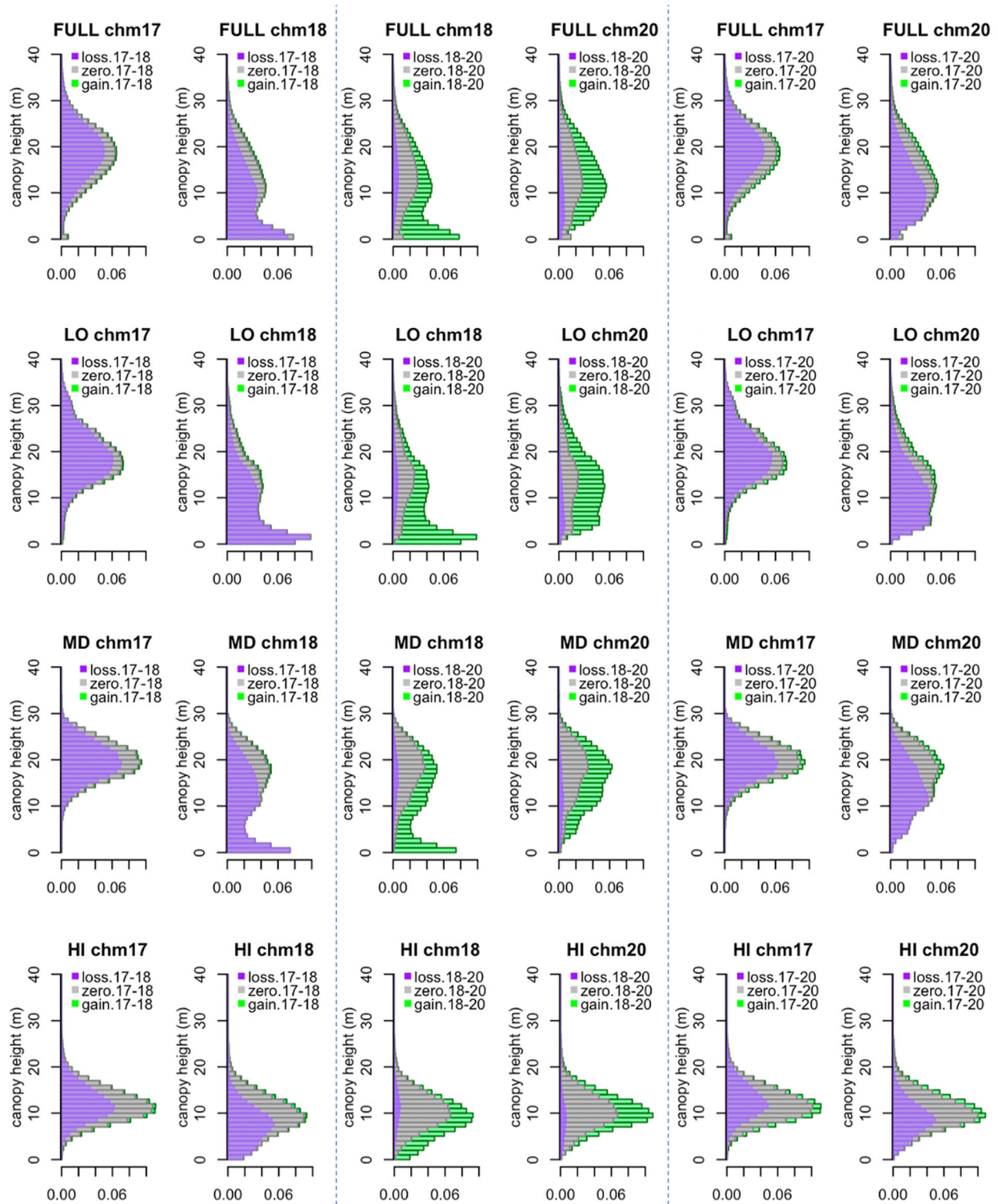
Figure 7. Canopy height distributions colored by change class, where paired figures in each time period illustrate the “from-to” movement of canopy material. Horizontal stacked bars in each 1-m height bin are colored according to the proportion of the study area associated with height loss (purple), height gain (green), and zero change (gray) categories for each time interval, 2017–2018 (left column), 2018–2020 (middle column), and 2017–2020 (right column).
