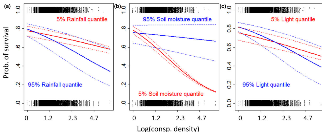
FIGURE 6 Seedling survival responses to the interactive effects of the number of conspecific seedlings and (a) rainfall, (b) soil moisture, and (c) understory light [Colour figure can be viewed at wileyonlinelibrary.com ]
