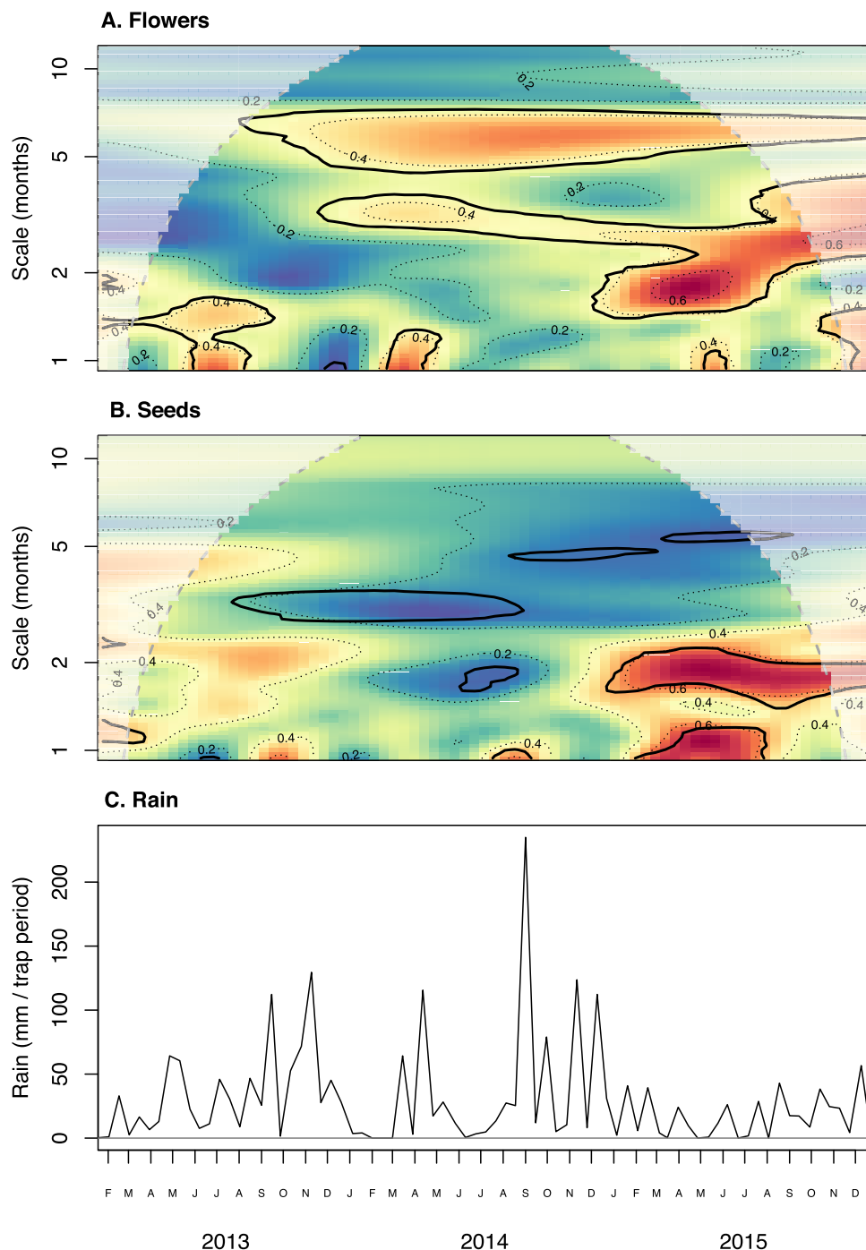
Figure 4. Synchronous versus compensatory dynamics of aggregate community (A) flowering and (B) seed rain, quantified with the wavelet modulus ratio (WMR). For comparison, (C) we show rainfall during biweekly observation intervals. The colors and dashed contours show WMR for reproduction across the course of the study (x-axis) and temporal scales (y-axis). Red indicates synchronous reproduction among species (high WMR) and blue indicates compensatory dynamics in reproduction (low WMR). Thick black contours bound points in time and scales where community reproduction was significantly synchronous or compensatory (non-parametric bootstraps, \alpha = 0.05 ). The shaded area indicates the cone of influence of edge effects, here defined as combinations of observation and temporal scale within one period of the beginning or end of the study.
