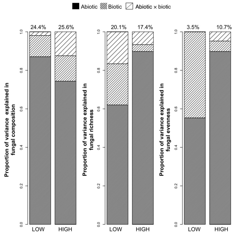
FIG. 4. Variance partitioning among abiotic (dark gray bars), biotic (narrow-hatched) factors, and their intersection (wide-hatched) that structure the community composition, richness, and evenness of soil fungi in low and high ILU. Total R^2 is indicated above each bar (%).
